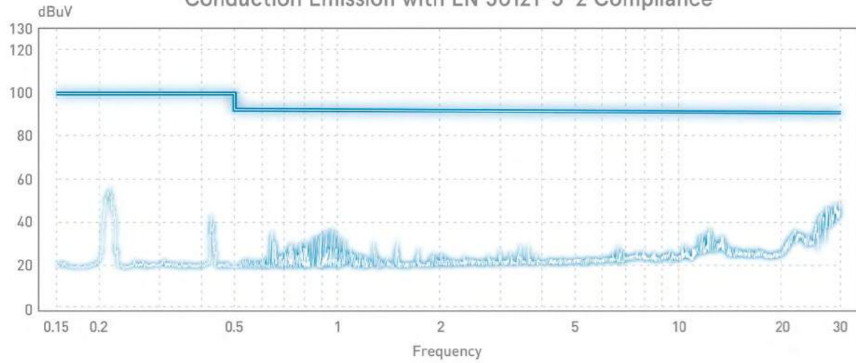
Conduction Emission with EN 50121-3-2 Compliance
