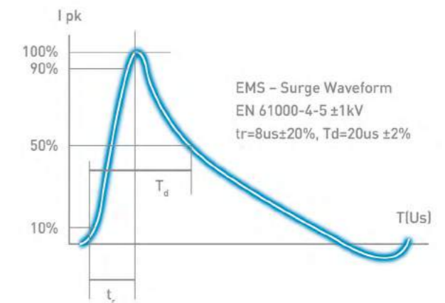
Electro Magnetic Susceptibility – EFT Waveform with EN 61000-4-5
