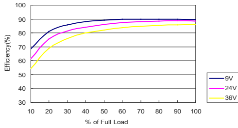
MJWI20-24S033 Efficiency vs Load Current
