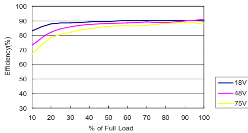
MJWI20-48D12 Efficiency vs Load Current
