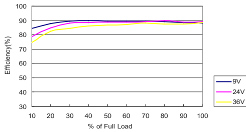
MJWI20-24D12 Efficiency vs Load Current
