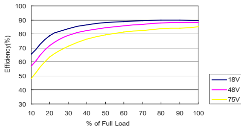
MJWI20-48S033 Efficiency vs Load Current
