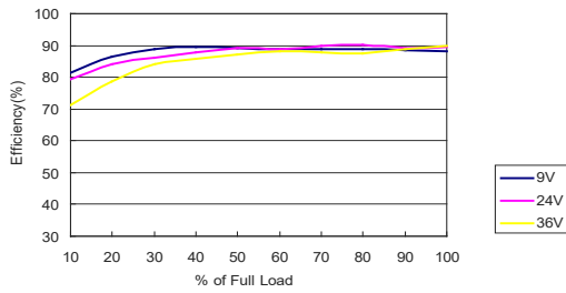
MJWI20-24S12 Efficiency vs Load Current
