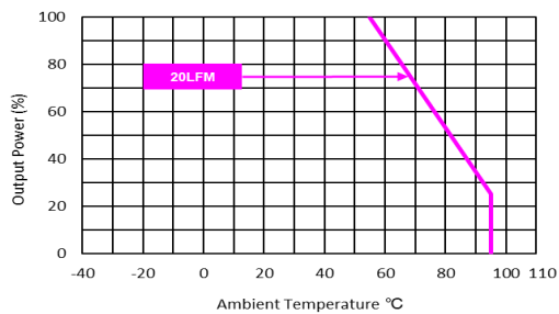
MDW15-12S12, MDW15-12S15, MDW15-12S24 MDW15-12D12, MDW15-12D15, MDW15-24S12 MDW15-24S15, MDW15-24S24, MDW15-24D12 MDW15-24D15, MDW15-48S12, MDW15-48S15 MDW15-48S24, MDW15-48D12, MDW15-48D15 Derating Curve without Heatsink
