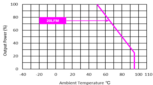
MDW15-12S051, MDW15-24S051, MDW15-48S051 Derating Curve without Heatsink
